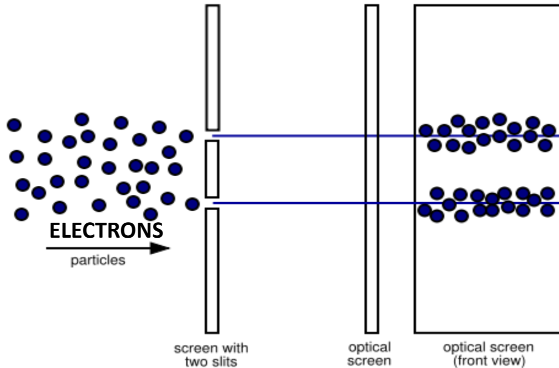
ELECTRONS SHOT THRU DOUBLE SLIT (EXPECTED RESULTS)
