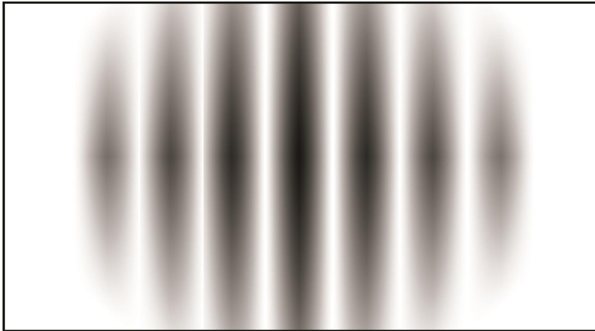
PATTERN WHEN NOT OBSERVED
